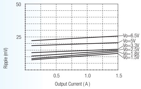
Ripple Vs Load (Vin=Max)
